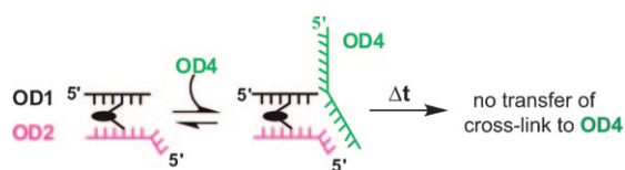
Scheme 3. Mere proximity is not sufficient for migration of DNA strand cross-linking. OD4 = 5'-d(CTTGAGATACTTTTTCTGCGCG-TCGTTGAAGAGGTA AAA).
