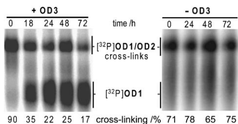
Figure 1. Cross-linking of OD1/OD2 by bisQMP dissipated in the presence, but not absence, of OD3 . The initial [ ^{32} P] OD1/OD2 cross-linking was formed indirectly by first treating [ ^{32} P] OD1 (3 \mu M) with bisQMP (60 \mu M) for 24 hours. OD2 (3 \mu M) was then added to the mixture, and incubation was continued for another 24 hours. Finally, OD3 (3 \mu M) was added to one portion of the mixture, and aliquots were removed for analysis after further incubation as indicated. Products were separated by denaturing polyacrylamide (15%) gel electrophoresis, quantified by phosphoimager of the indicated area and reported (%) relative to total DNA. OD1 = 5'-d(TGGTGTGGTGGT-TGGGTGTGTGGTGGGTGG), OD2 = 5'-d(TTTACTCTTCAACGCCGACCCACCAACCAACCAACCAACCA), OD3 = 5'-d(CTACTGACGTCTGTGTGGTGTGTGGGTGTGTGTGGTGGCGGTGAAGAGGTAAG).
